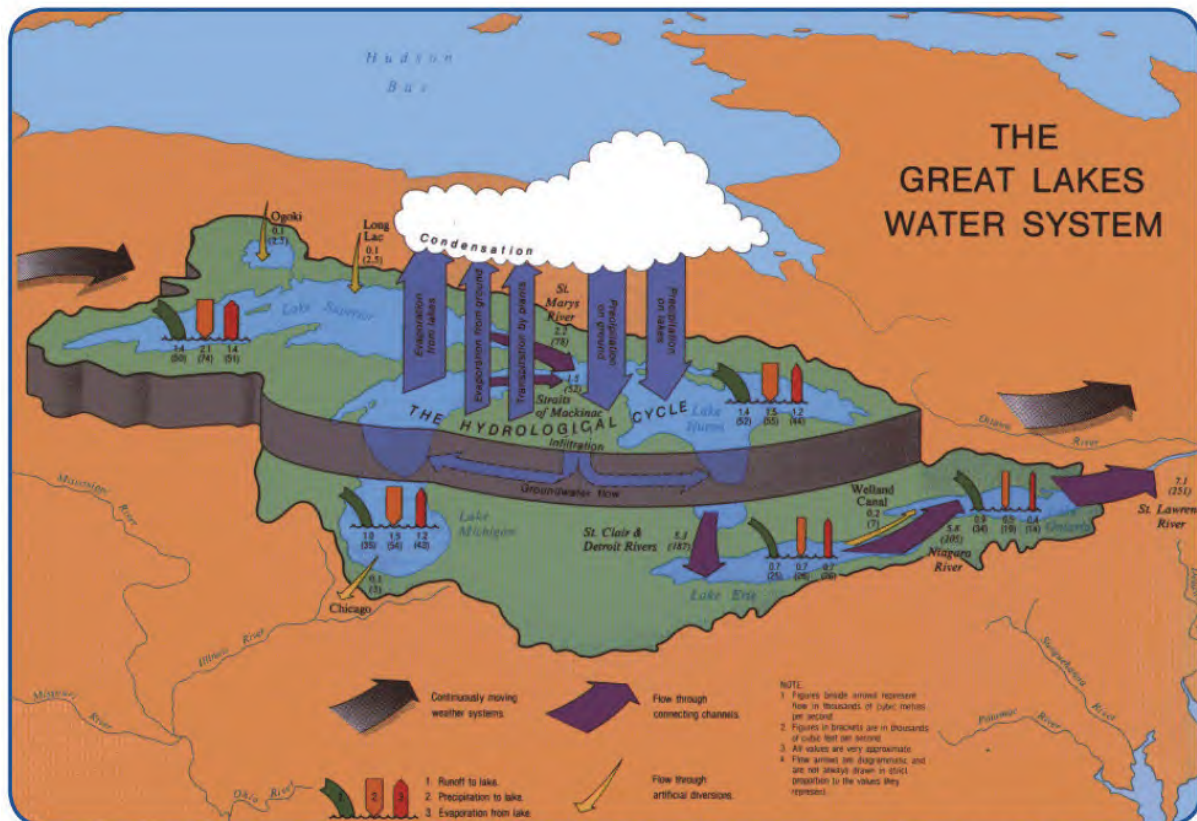
Figure 1. Schematic drawing of the Great Lakes Hydrologic Water System.
