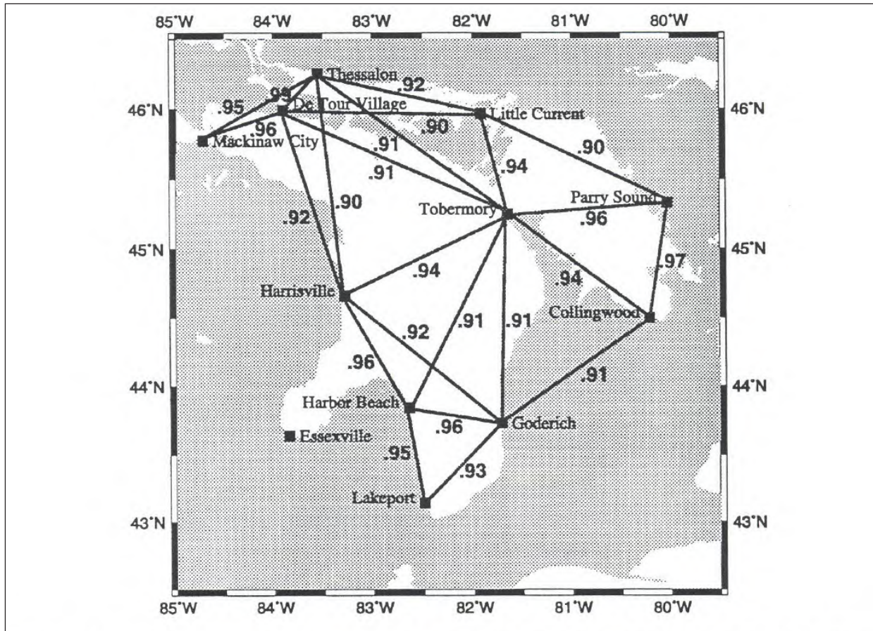
Figure 29. Lake Huron correlation coefficients from Zervas (1997). The new U.S. station at Alpena has replaced Harrisville subsequent to his study.
